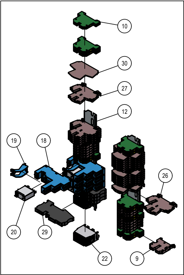
Detail A
